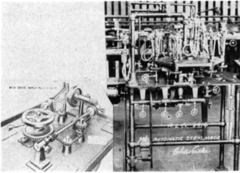
The first automatic stem machine, made at Westinghouse in 1914; the driving arrangements are shown left.
